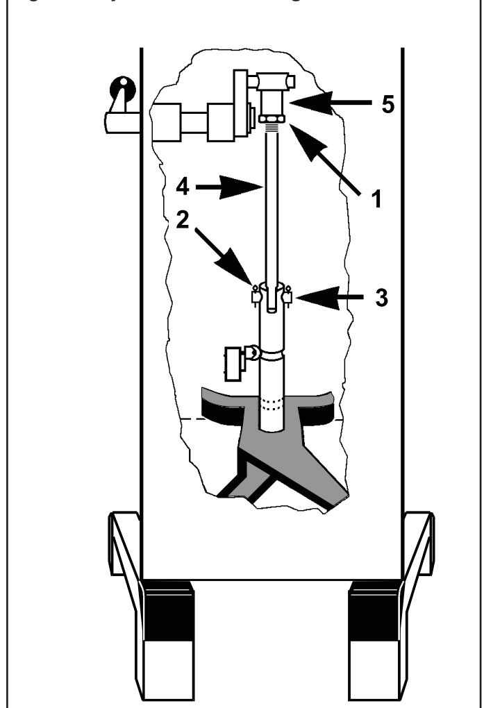
fig.7b Adjustment of bowl height:
