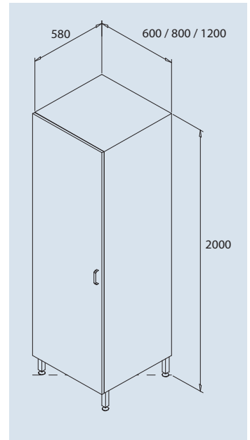
Floor cupboard, width 600 R/L, 800, 1200 mm
